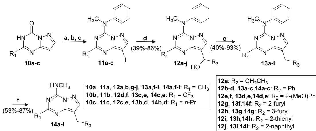
Fig. 5. (a) POCl_3 , DMAP, CHCl_3 , 120 °C, sealed tube, (b) N -methylaniline, CH_2Cl_2 , 25 °C, (c) NIS, CHCl_3 , reflux, (d) n -BuLi, R_3CHO , THF, −78 °C, (e) TMSCl, NaI, CH_3CN , (f) NH_2CH_3 , EtOH, 100 °C, sealed tube.
